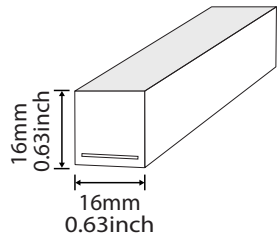
T1616 Profile
