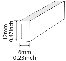
F0612 Profile
